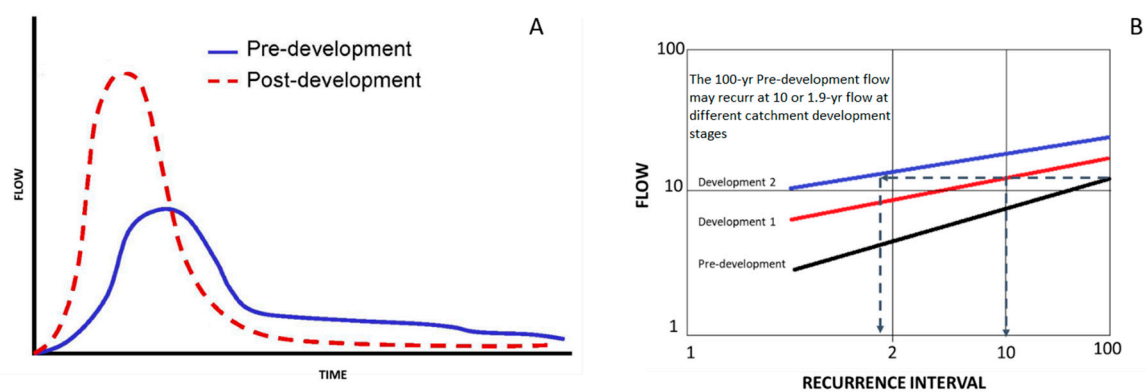
Figure 1. Effect of urban development on stormwater flow (A) and return frequency (B). With increasing urbanization, the recurrence interval of a 100-year flood can be reduced by one or more orders of magnitude, increasing the probability of risk to life and property.
